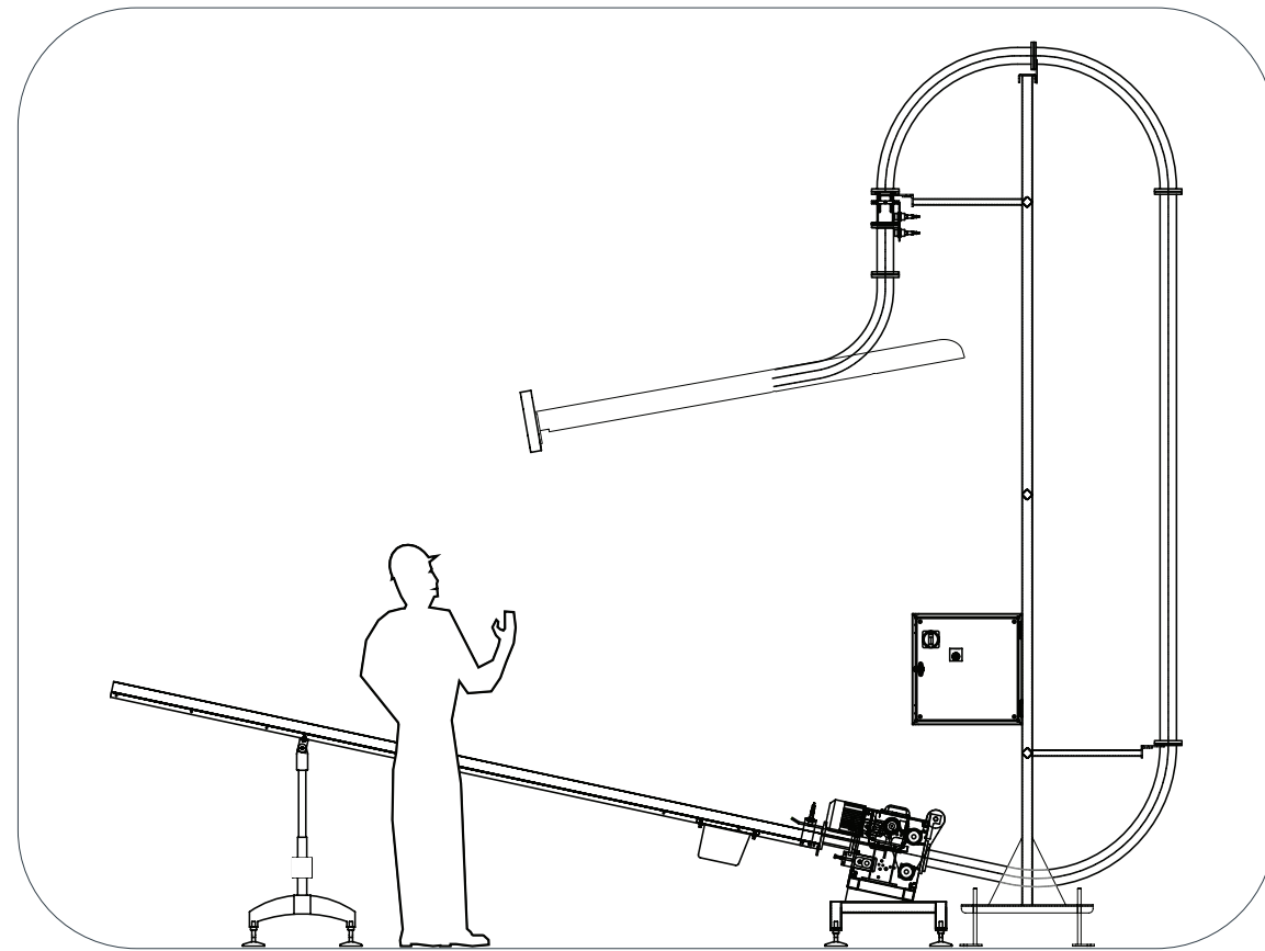
Drawing of Fleetwood Manual Can Lid Feeder with LLV Low Level V-Tray
